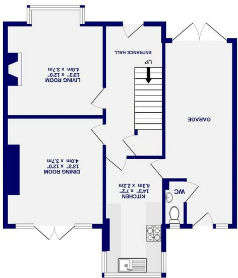
GROUND FLOOR 64.9 sq.m. (64.9 sq.m.) approx.
